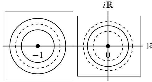
FIG. 1. Illustration of the contours for m = 2 : The two rectangles from left to right are \Omega_L and \Omega_R , the three contours around -1 from outside to inside are \Sigma_{2,L}^{\text{out}} , \Sigma_{1,L} , \Sigma_{2,L}^{\text{in}} respectively, the three contours around 0 from outside to inside are \Sigma_{2,R}^{\text{out}} , \Sigma_{1,R} , \Sigma_{2,R}^{\text{in}} respectively. \mathcal{S}_1 is the union of the three dashed contours, and \mathcal{S}_2 is the union of the three solid contours.
