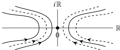
FIG. 2. Illustration of the contours for m = 2 : The three contours in the left half plane from left to right are C_{2,L}^{\text{in}}, C_{1,L}, C_{2,L}^{\text{out}} respectively, the three contours in the right half plane from left to right are C_{2,R}^{\text{out}}, C_{1,R}, C_{2,R}^{\text{in}} respectively. S_1 is the union of the three dashed contours, and S_2 is the union of the three solid contours.
